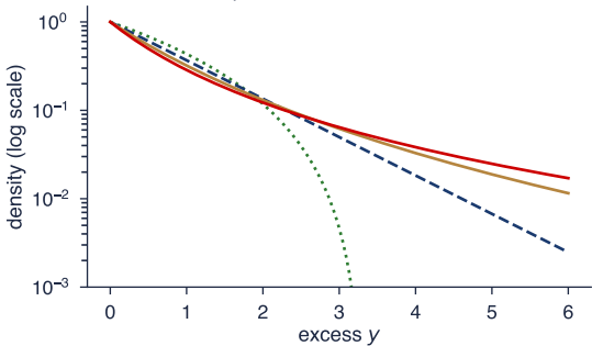
GPD densities, \beta = 1
