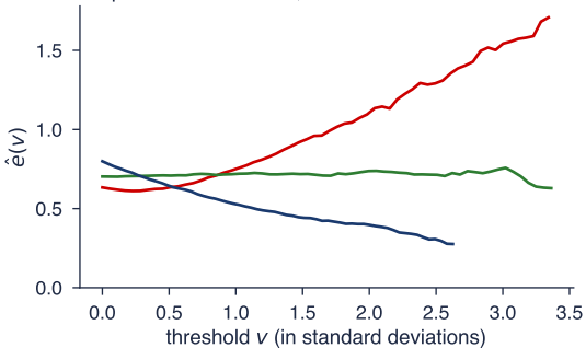
Empirical mean excess, 20000 draws each
