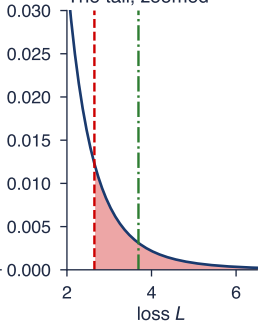
The tail, zoomed
