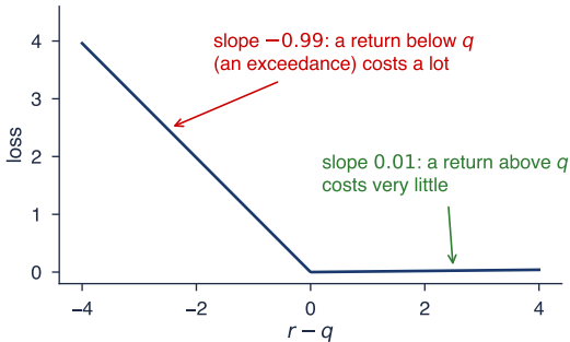
Pinball loss of the 1% quantile q
