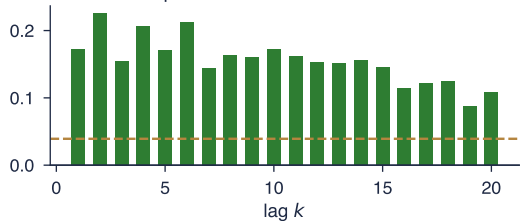
ACF of the squared returns
