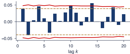
ACF of 2500 GARCH returns
