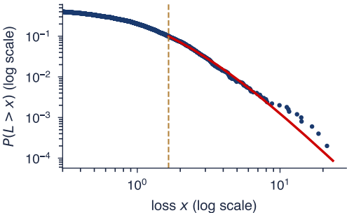
Tail of 5000 simulated losses
