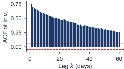
Long memory: slow decay
