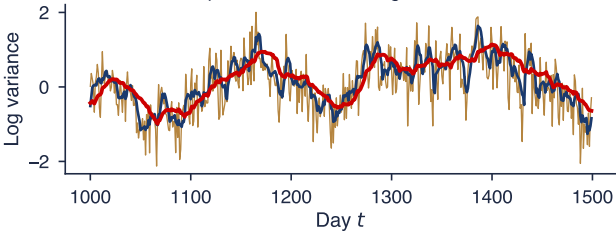
Simulated HAR process: three averages
