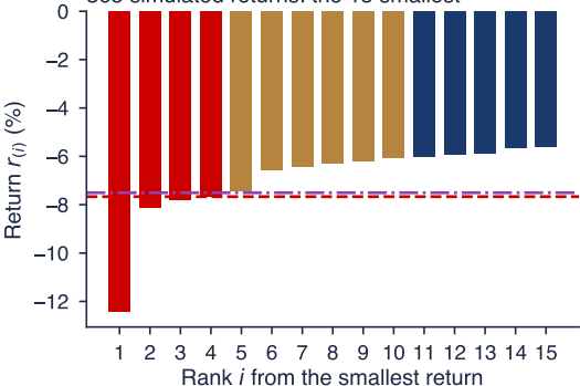
365 simulated returns: the 15 smallest
