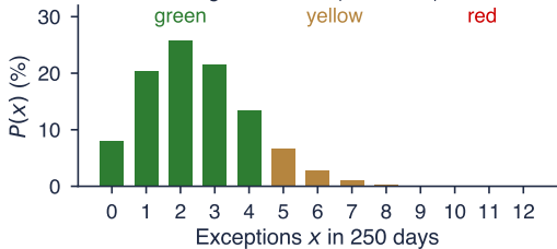
Basel traffic light: Binomial(250, 0.01)
