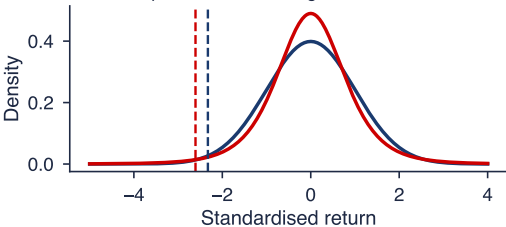
The 1% quantile: Normal against Student- t
