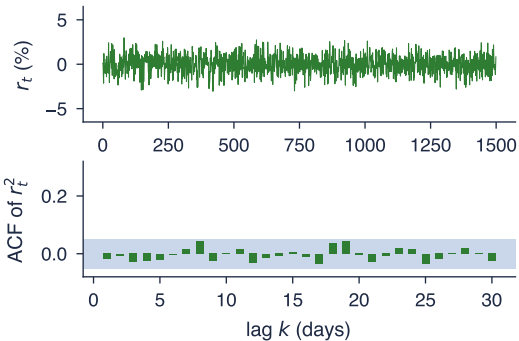
i.i.d. Normal returns (same variance)
