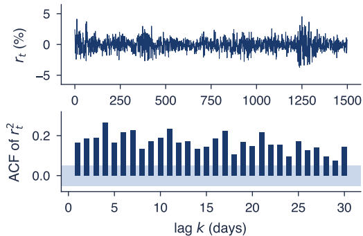
returns with clustering (same variance)
