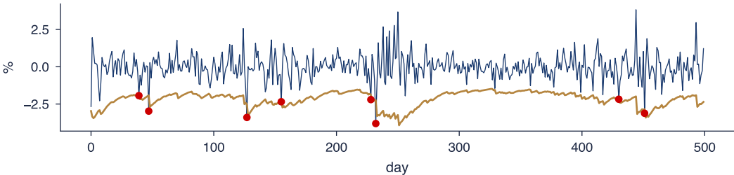
Simulated returns with heavy-tailed innovations; VaR computed with a Normal quantile
