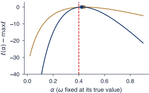
Log-likelihood of a simulated ARCH(1)
