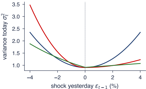
News impact curves ( \sigma_{t-1}^2 = 1 )
