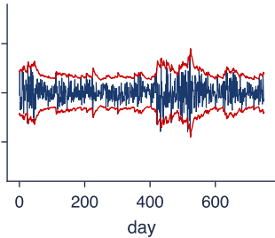
GARCH(1,1): \omega = 0.05, \alpha = 0.10, \beta = 0.85
