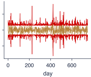
ARCH(1): \omega = 0.5, \alpha = 0.5
