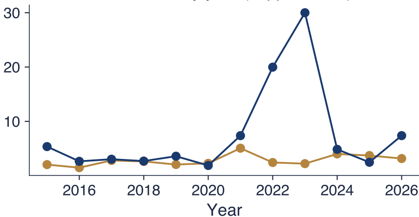
Student-t \hat{v} by year (capped at 30)
