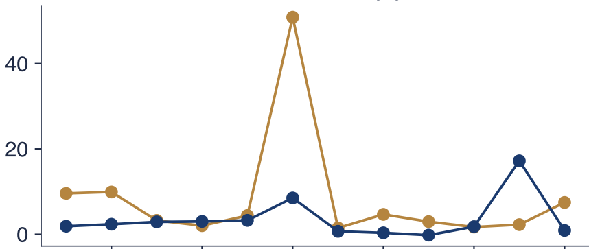
Excess kurtosis by year
