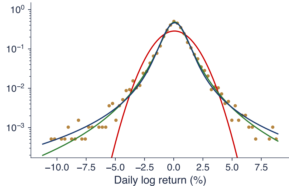
BET: \hat{\alpha} = 1.49
