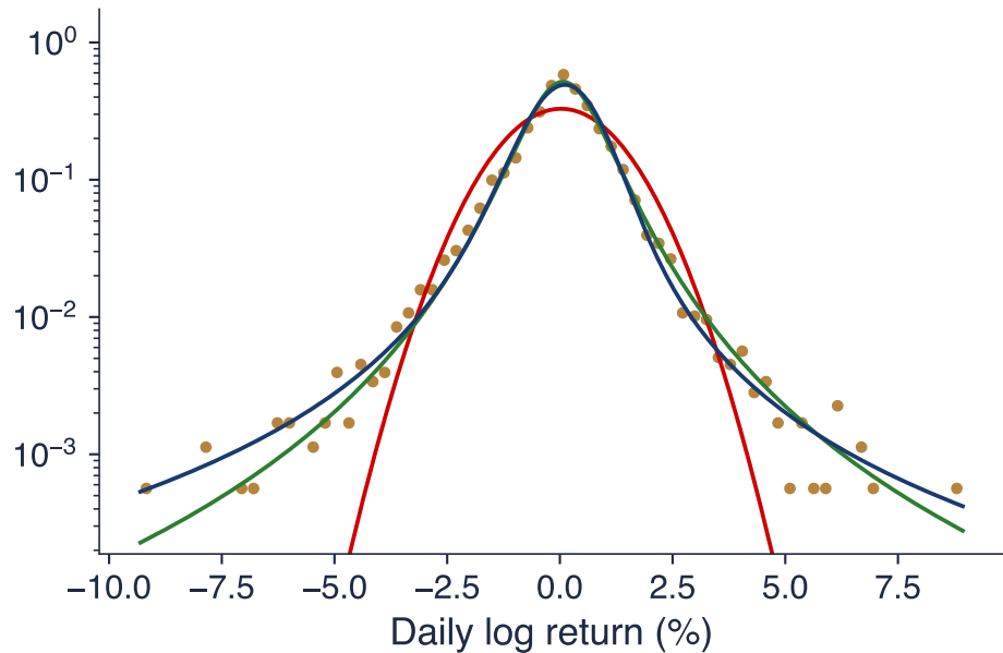
S&P 500: \hat{\alpha} = 1.54
