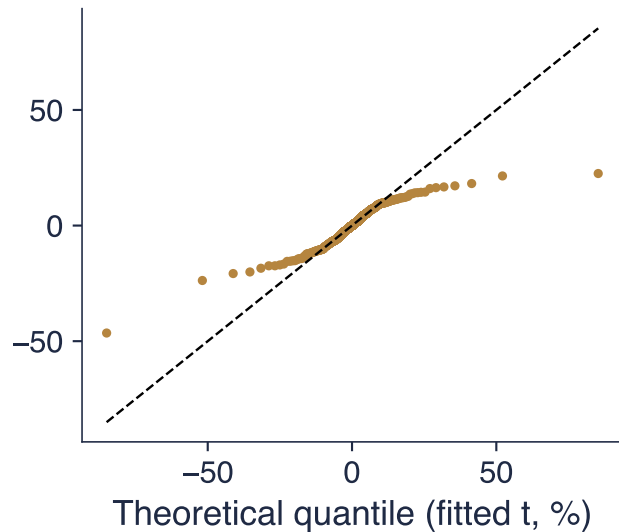
Bitcoin vs t(2.2)
