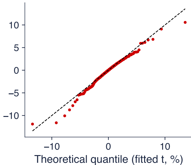
BET vs t(3.0)
