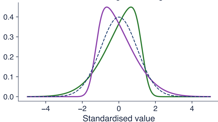
Skewness: a longer left or right tail
