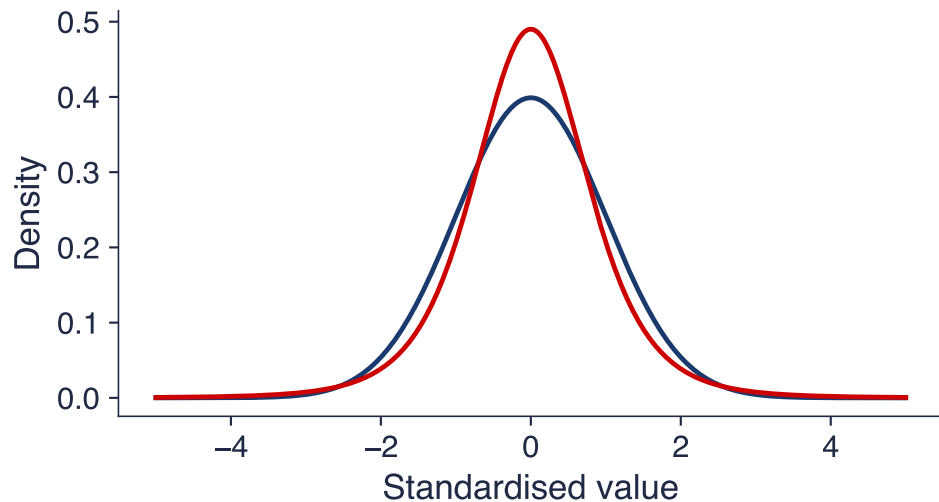
Kurtosis: taller centre, heavier tails
