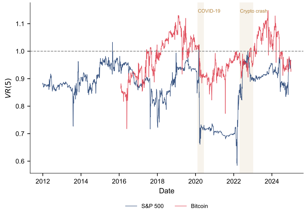
Panel B: Rolling VR(5), 500-day window
