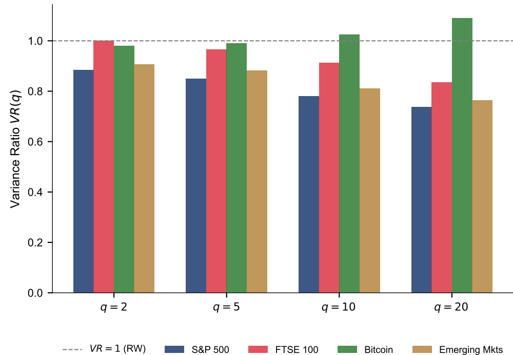
Panel A: Variance Ratio by Holding Period
