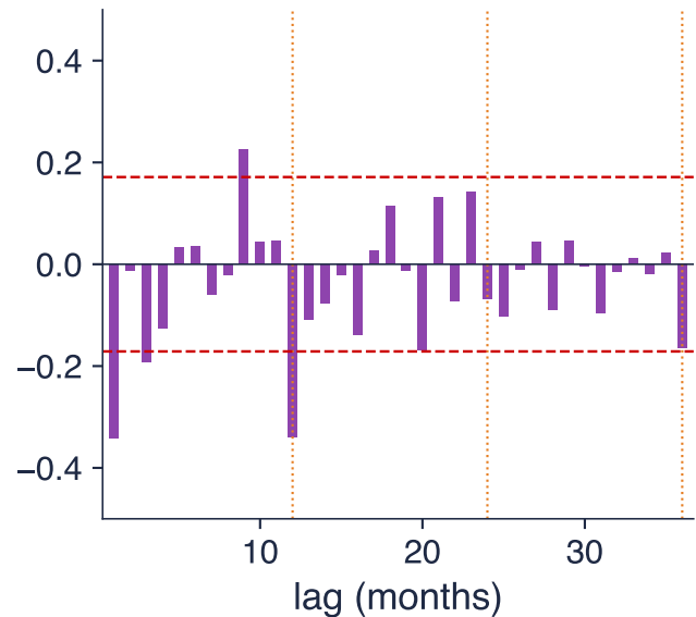
PACF of \Delta\Delta_{12}\ln y_t
