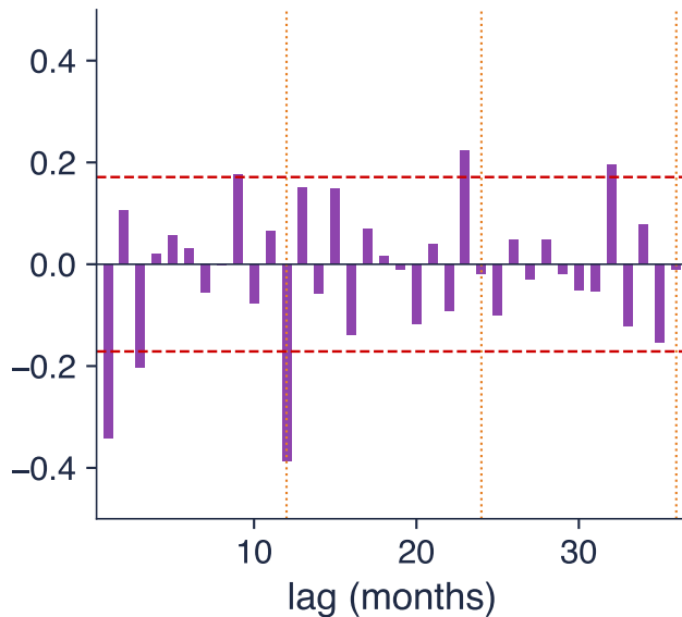
ACF of \Delta\Delta_{12}\ln y_t
