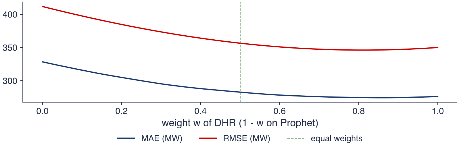
Combining DHR and Prophet: error as a function of the weight
