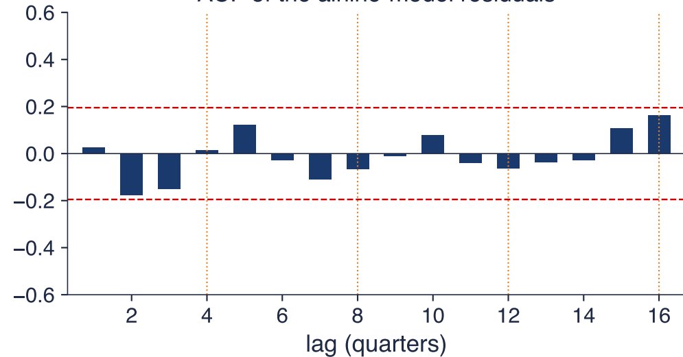
ACF of the airline-model residuals
