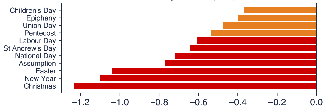
Holiday effects (GW)
