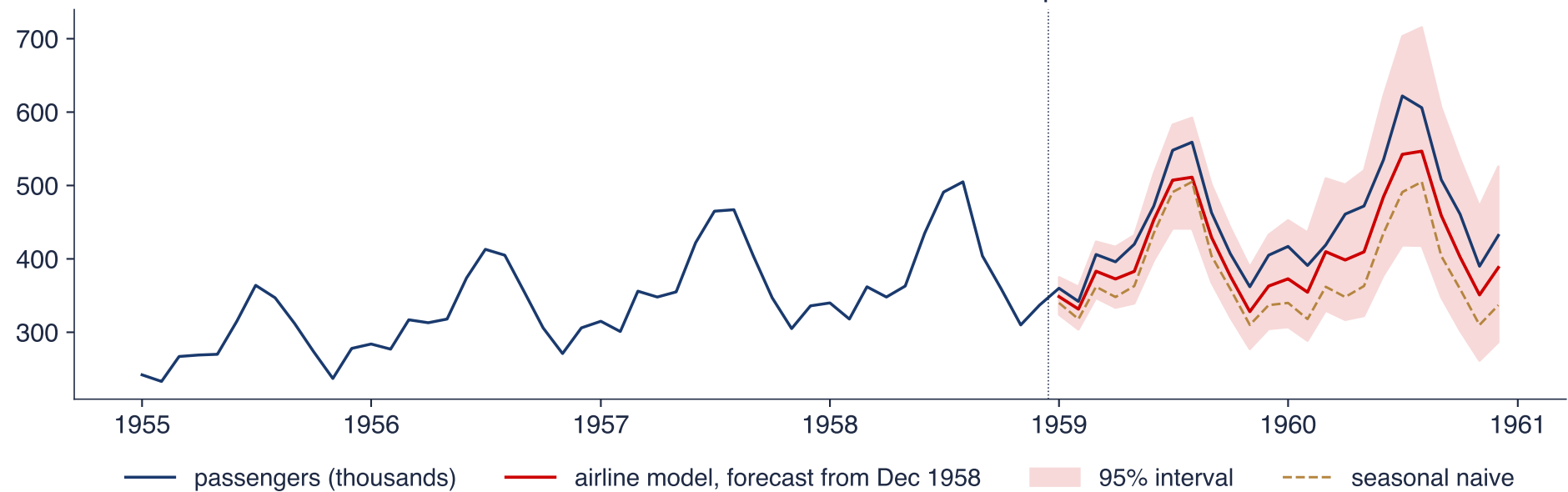
Airline model: 24 forecasts out of sample
