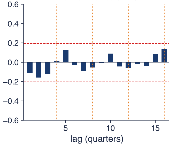
ACF of the residuals
