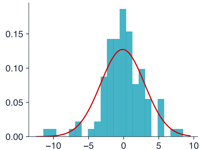
Distribution of the residuals
