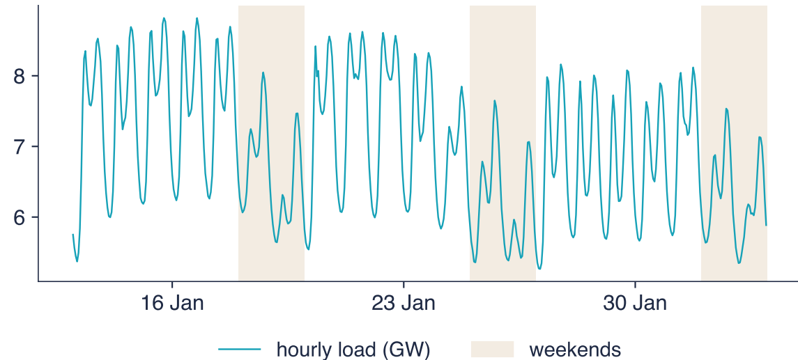
Hourly load, 13 January - 2 February 2025 (GW)
