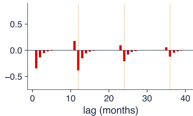
PACF: Airline: \theta = -0.4 , \Theta = -0.6
