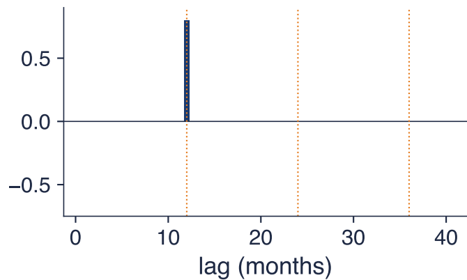
PACF: SAR(1) 12 , \Phi = 0.8
