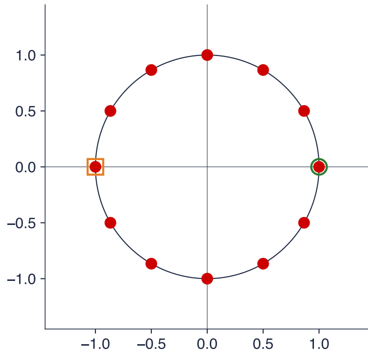
s = 12 : 12 roots of 1 - z^{12}
