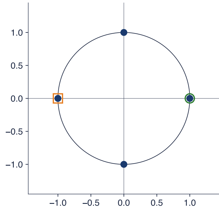
s = 4 : 4 roots of 1 - z^4
