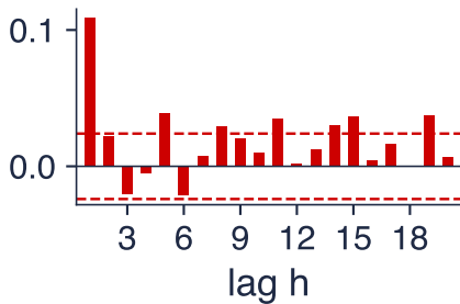
ACF of r_t
