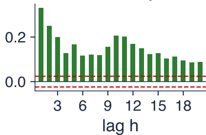
ACF of r_t^2
