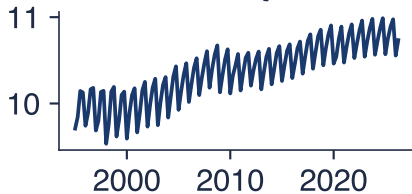
\ln Y_t
