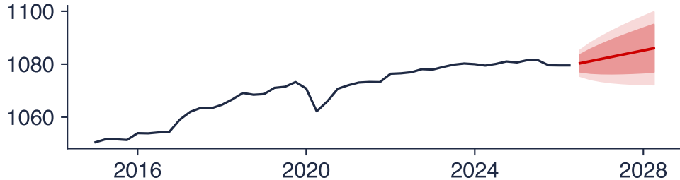
Romania: 100 ln real GDP and forecasts for 8 quarters
