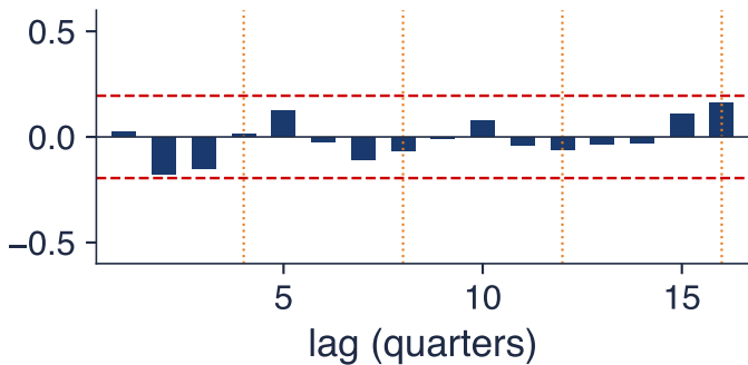
ACF of the airline-model residuals
