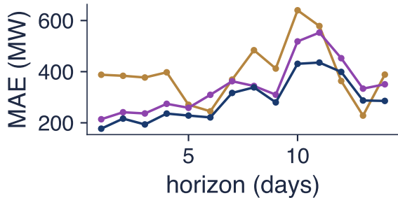
MAE by horizon
