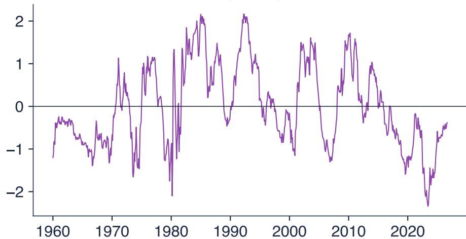
Residual of 10y on 1y (slope 0.83)
