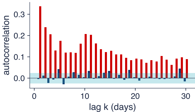
AR(1) with constant variance: residuals e(t)
