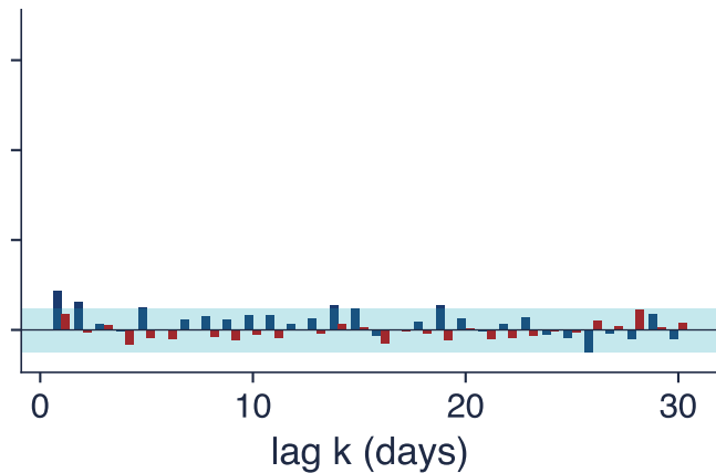
AR(1)-GARCH(1,1)-t: standardised residuals z(t)
