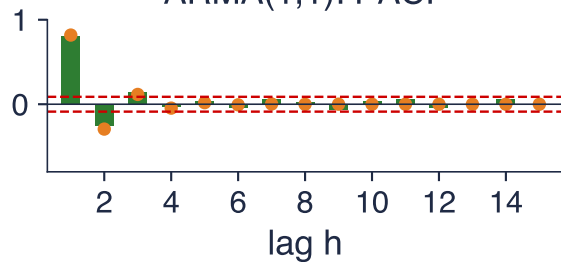
ARMA(1,1): PACF
