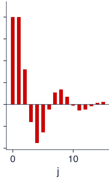
AR(2), \phi = (1.0, -0.6)
