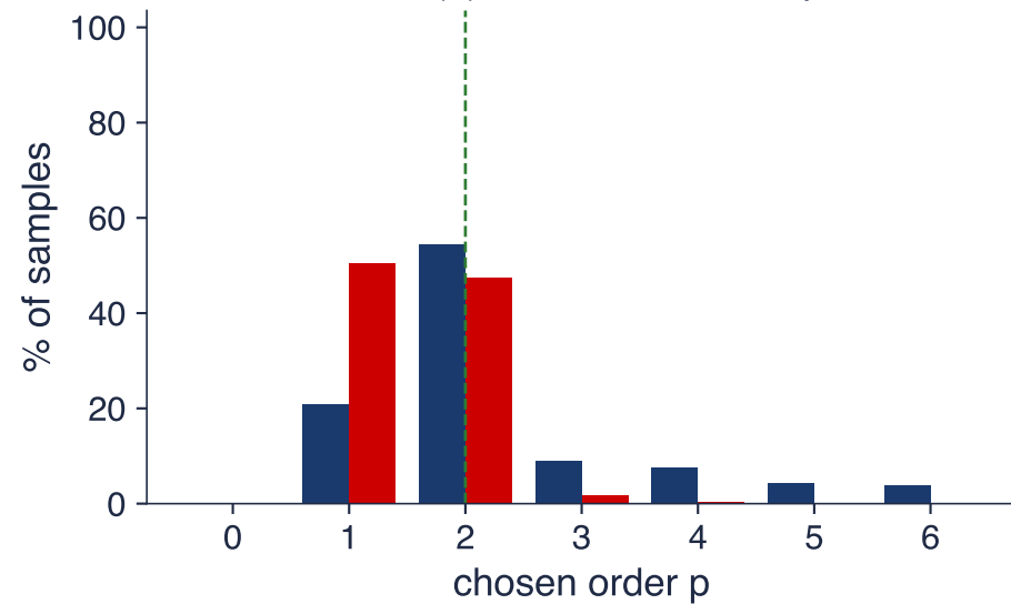
True AR(2), T = 100: 500 samples
