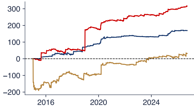
QLIKE(EWMA) - QLIKE(GARCH-t), cumulated
