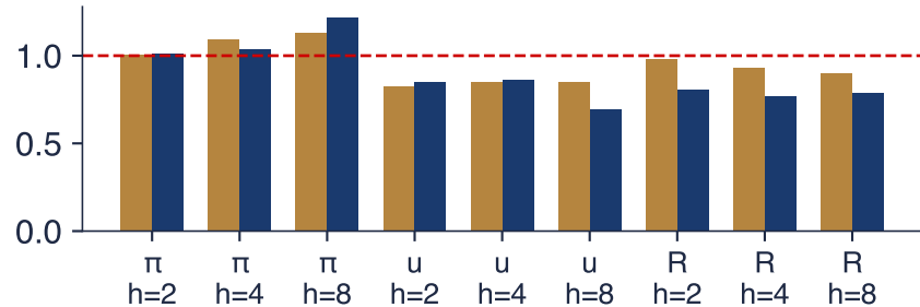
United States, forecasts for 1985-2000
