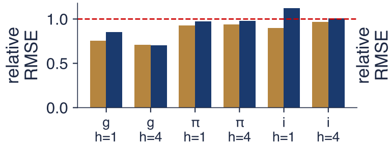
Romania, forecasts for 2015-2026
