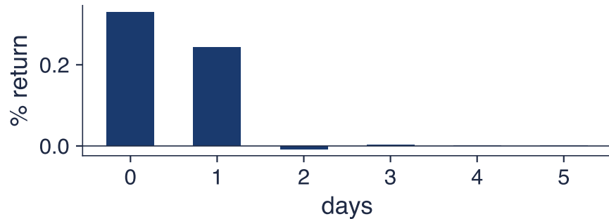
Generalised impulse response, VAR(1)
