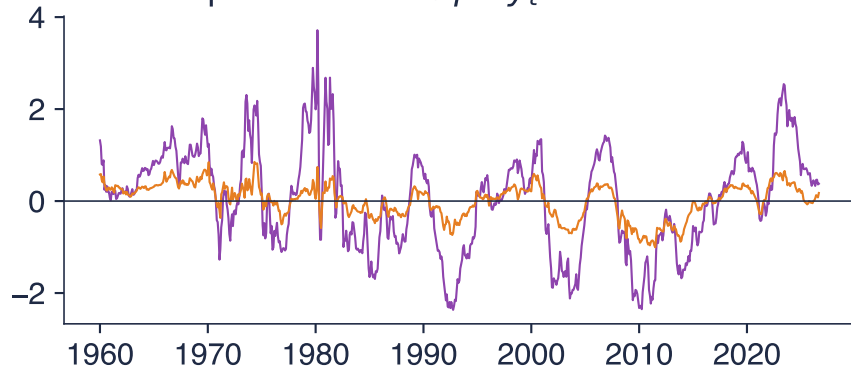
Equilibrium errors \hat{\beta}^\top y_t of the VECM
