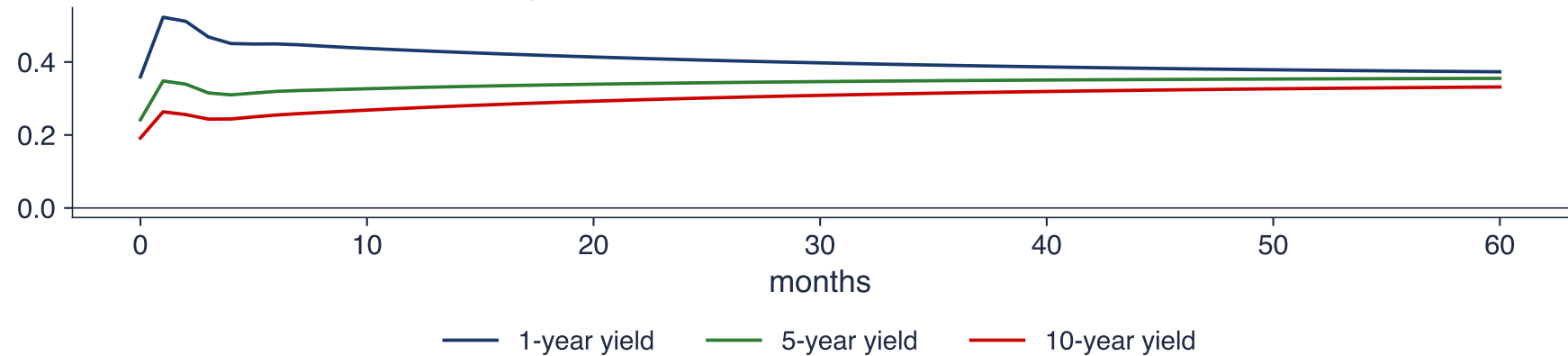
Response (percentage points) to a one-standard-deviation shock to the 1-year yield
