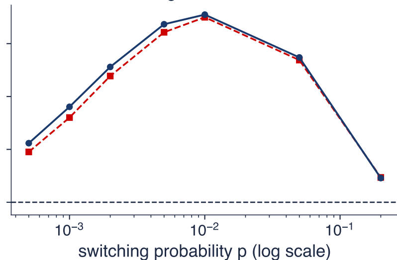
Markov switching between means 0 and 1
