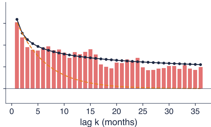
BET: d = 0.36 (ML), 0.39 (LW), 0.44 (GPH)
