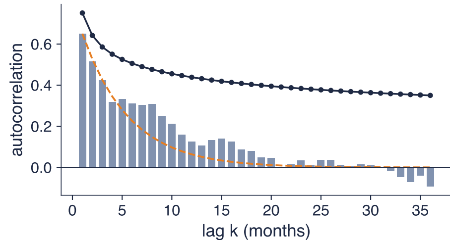
S&P 500: d = 0.40 (ML), 0.41 (LW), 0.37 (GPH)
