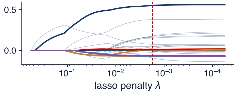
lasso: coefficients drop to exactly zero
