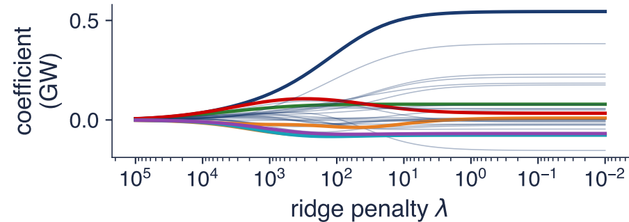
ridge: all coefficients shrink smoothly
