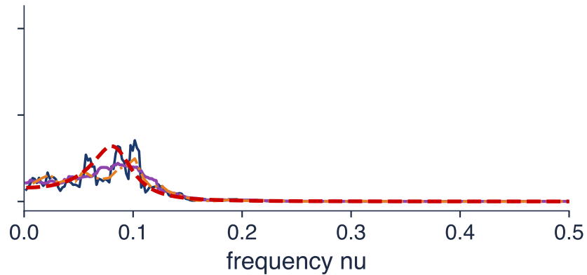
Smoothed estimates
