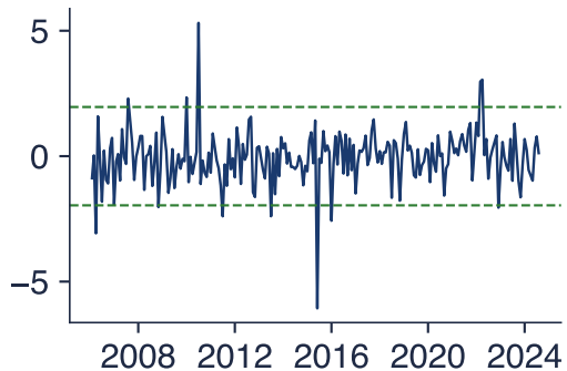
residuals over time
