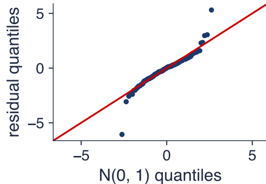
QQ plot against N(0, 1)
