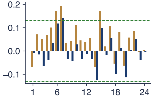
ACF of the residuals
