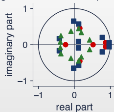
Eigenvalues of the companion matrix
