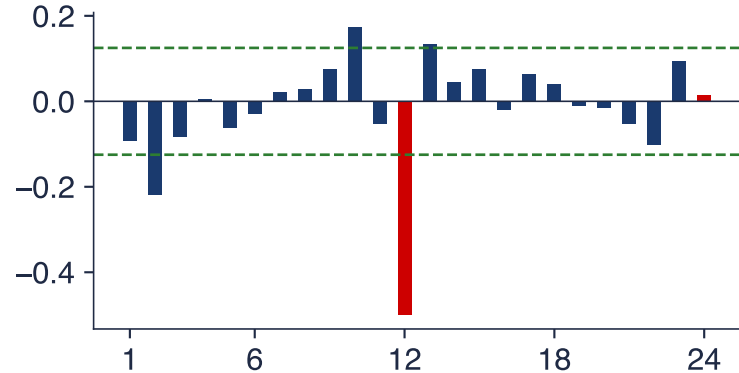
ACF of \Delta\Delta 12 \ln IP
